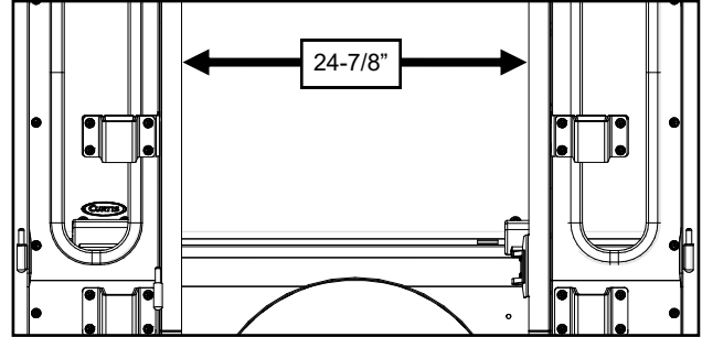
Fig. 11.1 (Measure Rear Legs Left to Right)
