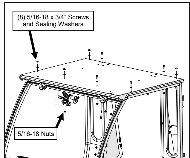
Fig. 10.1 (Install Roof)
