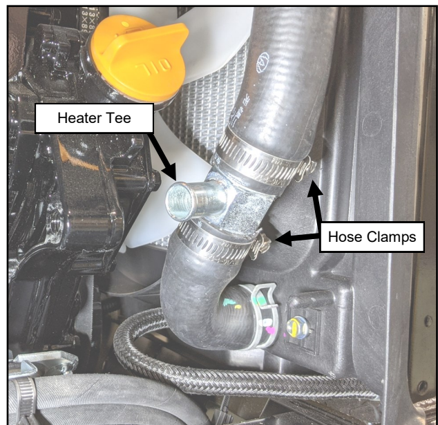
Fig. 18.3 (Tee Fitting)
