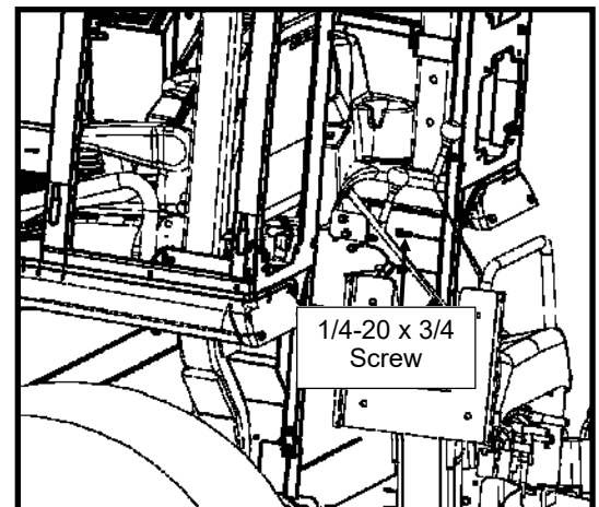
Figure 7.3b: Right Rear Corner Filler
