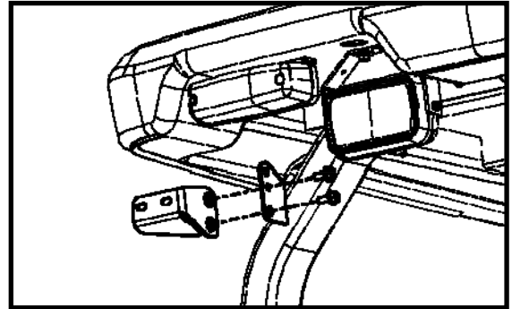
Figure 5.4: Upper Rear Mount
