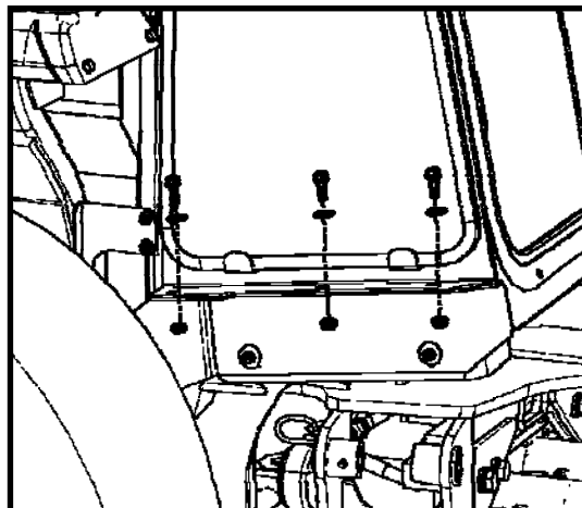
Figure 18.5: Fasten Backhoe Cab
