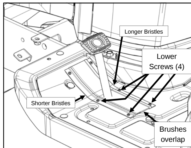
Figure 2.1 (Brake Pedal Brushes)
