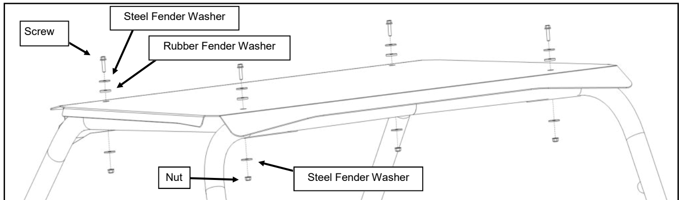
Fig. 1.2 (Roof Hardware)
