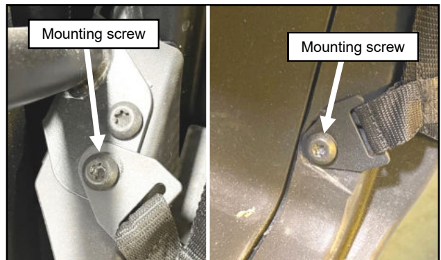
Fig. 1.3 (Remove Left Net Mounting Screws)
