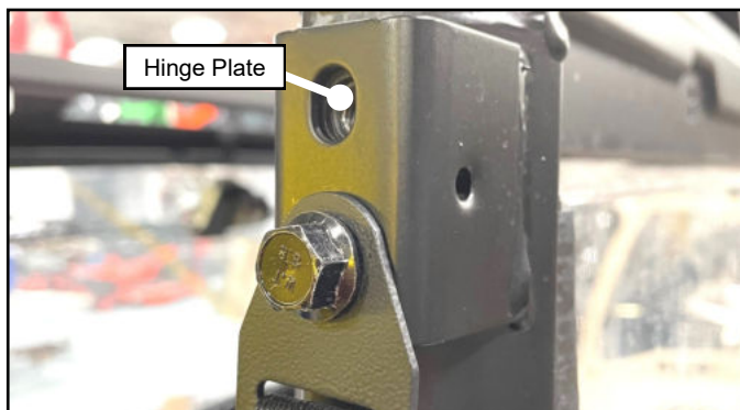
Fig. 1.5 (Remove Top Left Net Mounting Screw)
