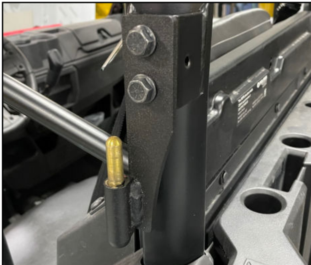
Fig. 2.3 (Lower Hinge Pin, Left)
