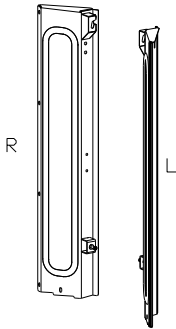
REAR LEG ASS'Y. RIGHT P/N: 8SV-GC1708R-R3 LEFT P/N: 8SV-GC1708L-R3
