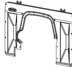
COWL ASS'Y. P/N: 8SV-GC179505-R3
