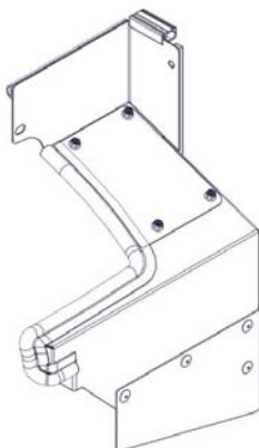
LOWER REAR FILLER, RIGHT P/N: 8SV-KL47-21-R
