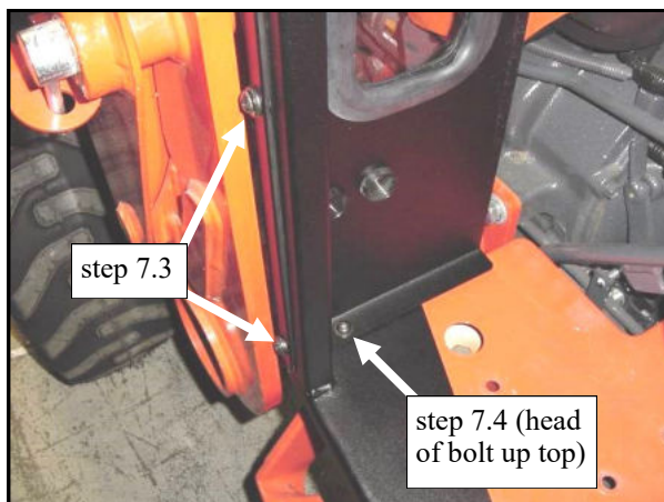
Fig. 7.3 (view from left rear side of tractor)
