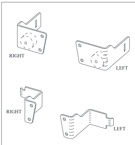
KIT SERVICE PART NO. AND DESCRIPTION: LOWER ROLL BAR MOUNT SET P/N: 8SV-110-00012
