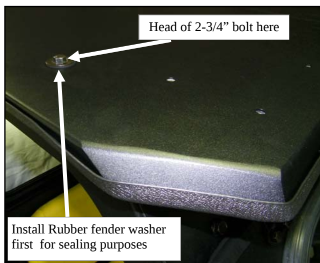
Fig. 5.2 (view of passenger's side front corner)
