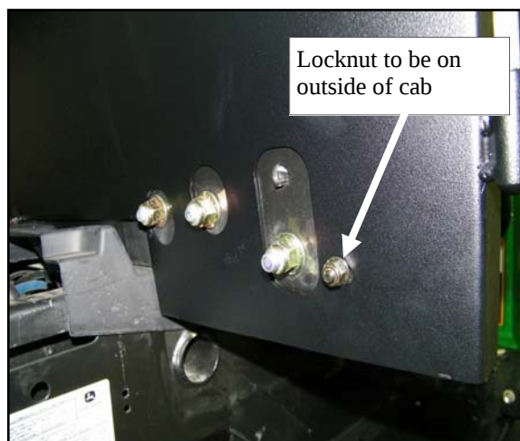
Fig. 1.4 (view from rear of passenger's side)
