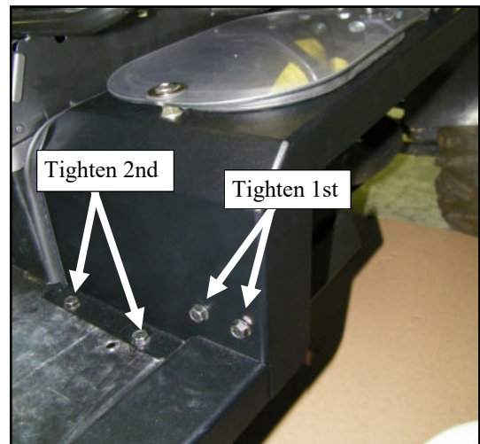
Fig. 9.2 (view of fuel tank shroud)
