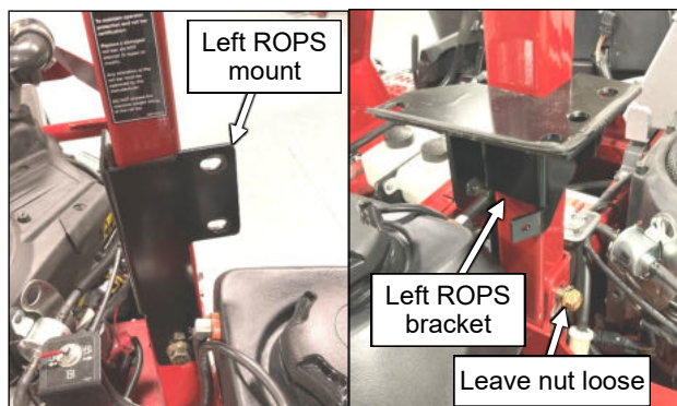
Fig. 3.3 (Install left side ROPS mount)
