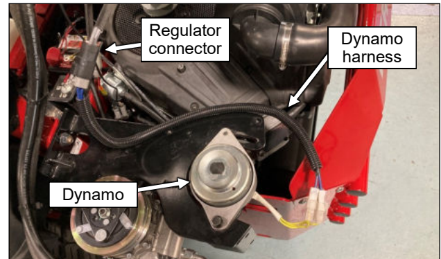
Fig. 6.9 (Dynamo connections)
