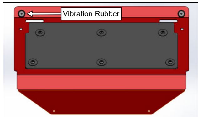
Fig. 2.1.4 (New Floorboard)
