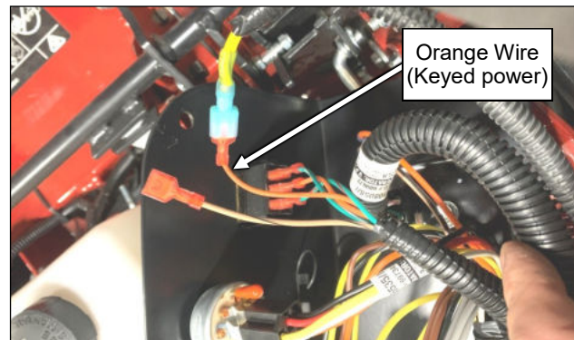
Fig. 6.3 (Keyed power connection, option 1 of 2)
