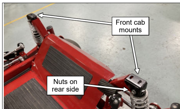
Fig. 3.5 (Install front cab mounts)
