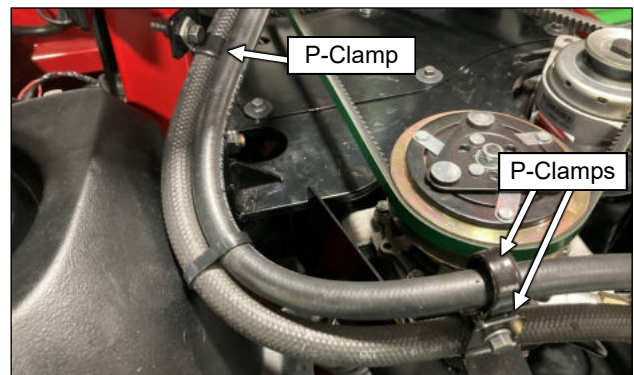
Fig. 9.2 (A/C hose P-clamps)
