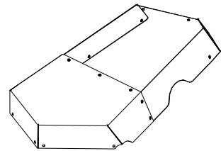
FLYWHEEL SHROUD P/N: 8SV-113-00342
