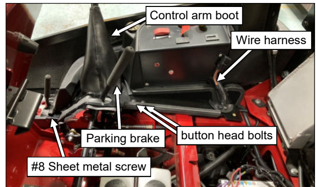
Fig. 10.9 (Right side under-seat panel)
