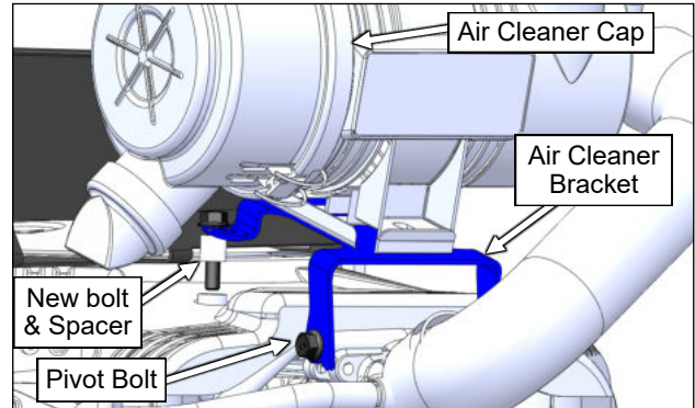
Fig. 8.1 (36HP Air Cleaner)
