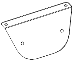
REGULATOR MOUNT BRACKET P/N: 8SV-SM-02530
