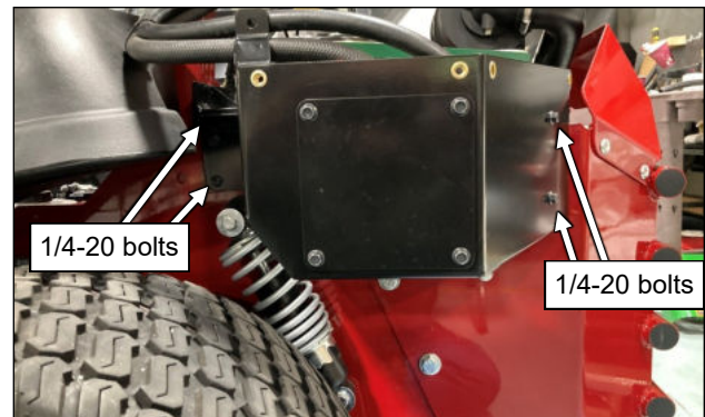
Fig. 9.1 (Compressor Debris Cover)
