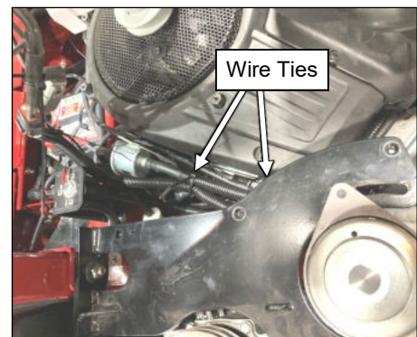
Fig. 6.12 (Secure compressor wires)
