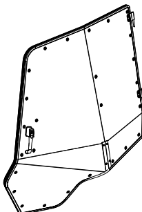
SIDEFAME ASSEMBLY, RIGHT P/N: 8SV-109-00027-R
