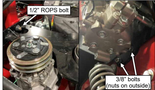
Fig. 5.1 (A/C compressor bracket)
