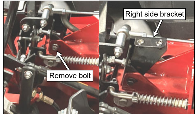
Fig. 10.7 (Right side inner panel bracket)
