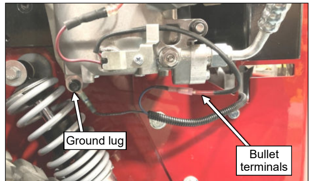
Fig. 6.7 (Compressor connections)
