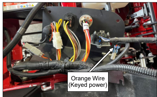
Fig. 6.3a (Keyed power connection, option 2 of 2)
