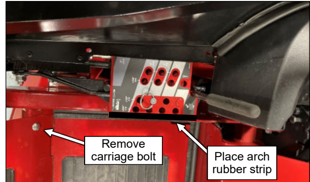
Fig. 10.1 (Deck control foam seal)
