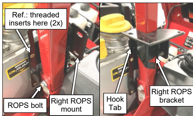
Fig. 3.1 (Install right side ROPS mount)
