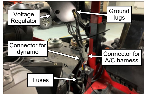
Fig. 6.8 (Voltage Regulator Connections)
