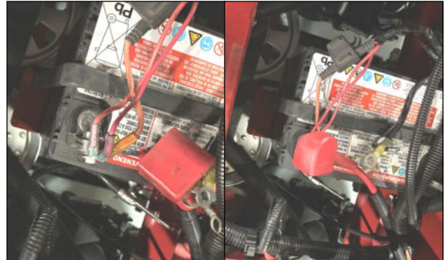
Fig. 6.4 (Positive wire connections)
