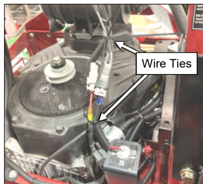
Fig. 6.11 (Secure regulator wires)
