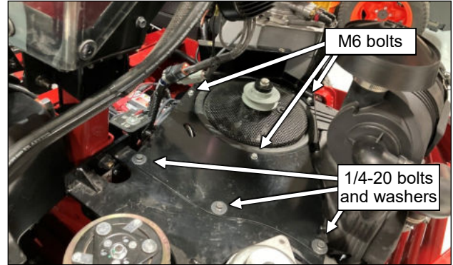
Fig. 7.1 (Flywheel shroud mount)
