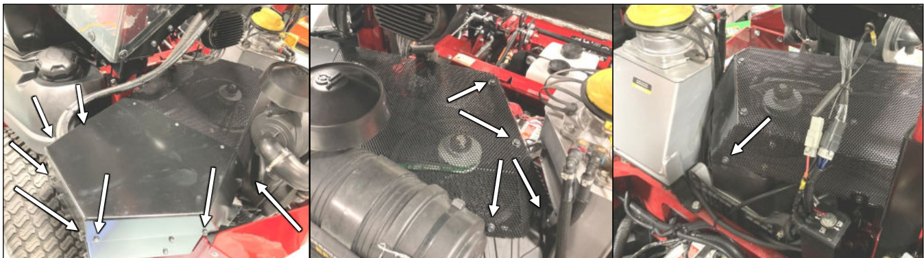
Fig. 9.3 (Flywheel shroud)
