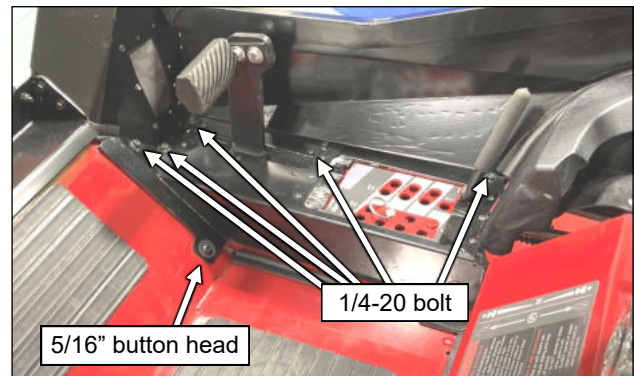
Fig. 10.3 (Deck Control Cover)
