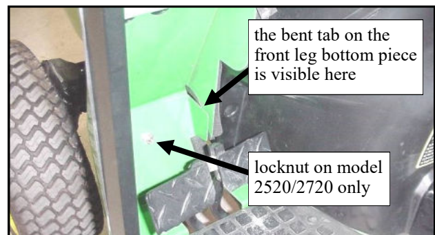
Fig. 8.1.3 Left Front Leg (models 2520/2720 shown)
