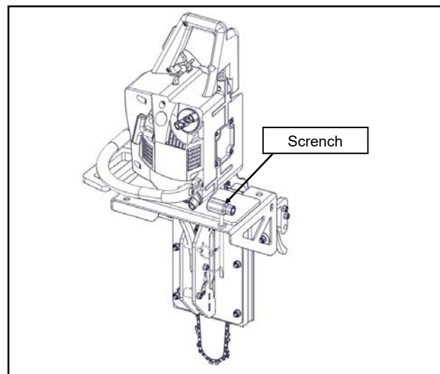
Fig. 8 (installing Srench)
