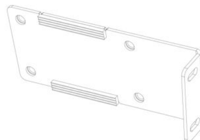
HINGE KIT, TOP & BOT, RIGHT P/N: 8SV-HKWTB-R
