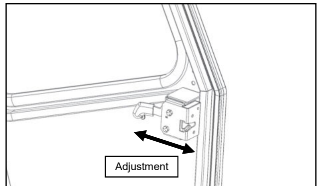
Fig. 18.3b (Door Latch Adjustment)
