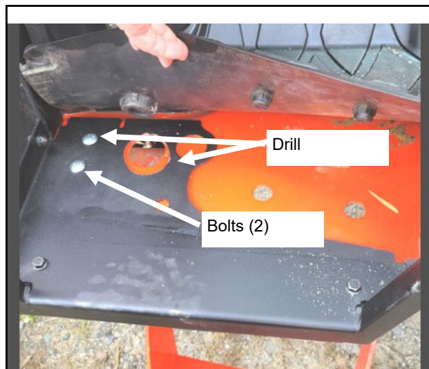
Fig. 4.1 (Modify floorboard mounts)
