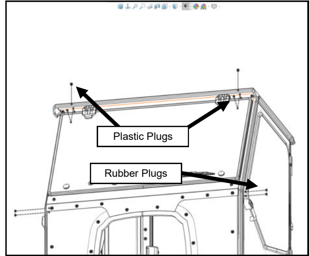
Fig. 19.1 (Install Plugs)
