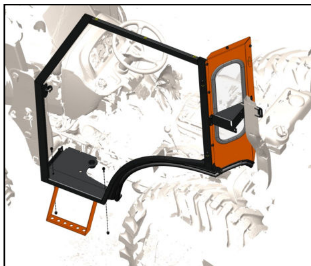
Fig. 4.2 (Side Frame)
