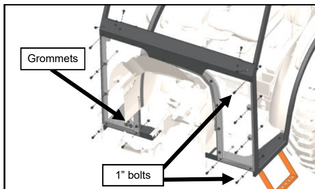
Fig. 5.1 (Cowl)
