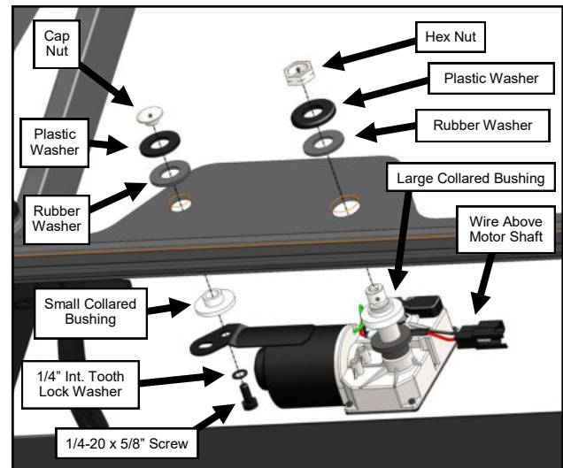
Fig. 11.1 (Wiper Motor)
