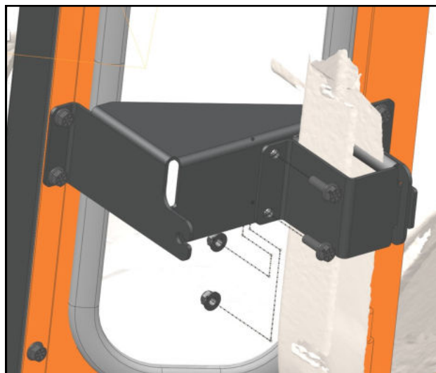
Fig. 4.3 (ROPS Bracket)
