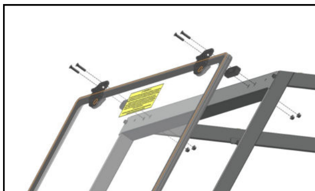
Fig. 7.1 (Windshield Hinges)
