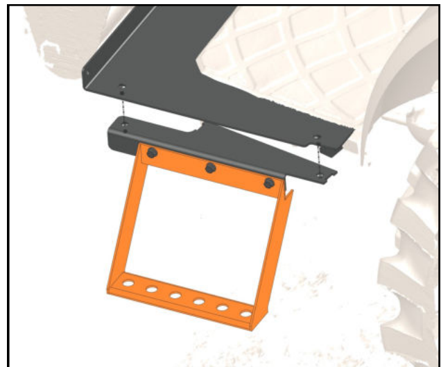
Fig. 2A.3 (Step Adapter)
