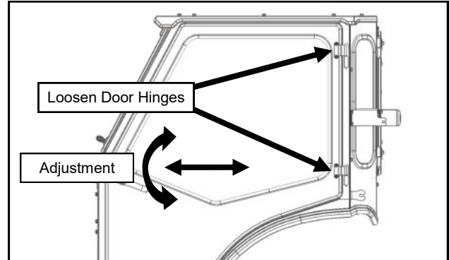
Fig. 18.3a (Door Hinge Adjustment)
