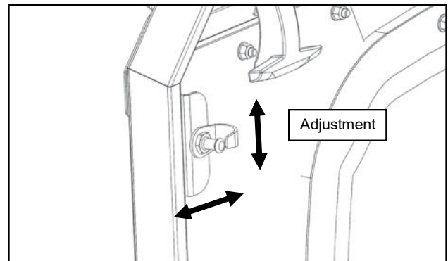
Fig. 18.4 (Striker Pin Adjustment)
