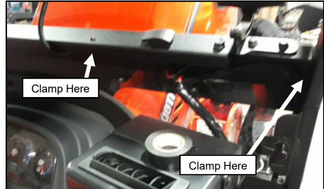
Fig. 13.3 (Wiring at Cowl)
