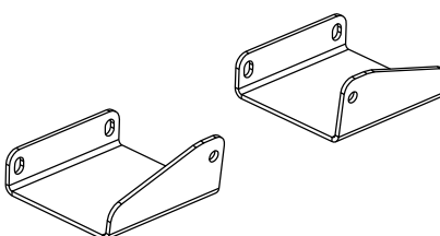
ROPS LOWER BRACKETS, (SET OF LEFT / RIGHT) P/N: 8SV-SM-01021
