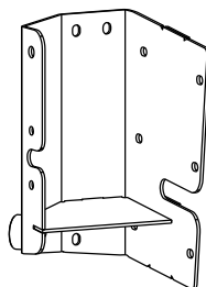
ROPS BRACKET, LOWER, LEFT P/N: 8SV-110-00045-L
